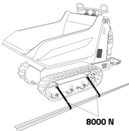
fig. 32 Anchoring points for transport
